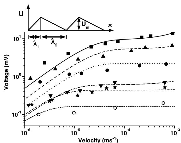
Fig. 2. Induced Voltage (V) as function of liquid velocities, for water (●); methanol (○), mixture of water:glycerol (75:25) (★); Water:glycerol (88:12) (▼); 0.6 M HCl (▲), and 1.2 M HCl (■). The ratios for the water-glycerol mixtures are by volume. Lines show the best fit of the data to Eq. 2. Inset shows a schematic of asymmetric ratchet potential.
