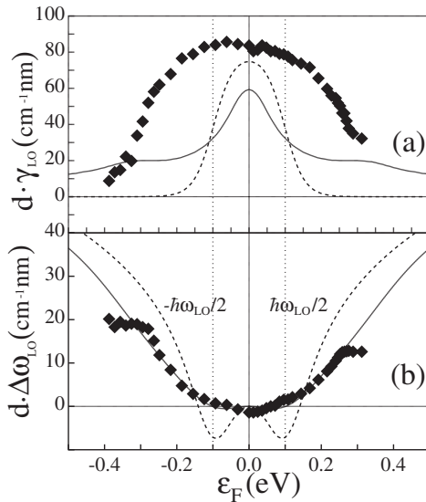
FIG. 3. G^- peak in metallic tubes: (a) Linewidth ( \gamma_{\text{LO}} , FWHM) and (b) frequency shift ( \Delta\omega_{\text{LO}} ) as a function of the doping. The Fermi energy ( \epsilon_F ) is zero at the charge neutrality point. \gamma_{\text{LO}} and \Delta\omega_{\text{LO}} are multiplied by the tube diameter ( d ) to obtain a universal behavior. Diamonds are measurements ( L1 line). Lines are calculations done by considering (full line) or not considering (dashed line) an inhomogeneous fluctuation of \epsilon_F . \omega_{\text{LO}} is the frequency of the LO phonon.
