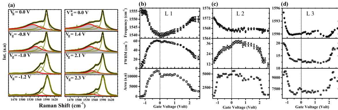
FIG. 2 (color online). (a) Tangential Raman modes of SWNTs recorded using an excitation energy of 1.96 eV at several V_g . The open circles (dark yellow) show the raw Raman spectra, and the black lines are the fitted one. The shaded Raman spectra show the LO phonon component of the metallic nanotubes. V_g dependence of (b) L1 , (c) L2 , and (d) L3 modes: Frequency (top panel), FWHM (middle panel), and total integrated area (bottom panel).
