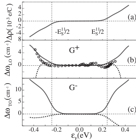
FIG. 4. G^+ and G^- peaks in 1.6 nm semiconducting tubes: (a) Theoretical charge doping per C atom. (b),(c) Frequency shift ( \Delta\omega_{\text{LO}} , \Delta\omega_{\text{TO}} ) as a function of the Fermi energy ( \epsilon_F ). Open dots are measurements ( L3 line). Dotted lines are adiabatic calculations (BOA). Full lines are our most accurate theoretical results that take into account dynamical effects (TDPT). Vertical lines are the theoretical position of the first van Hove singularities.
