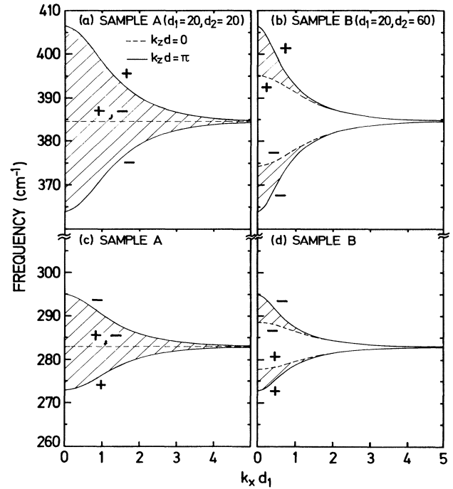
FIG. 3. Calculated interface modes from Eq. (1). The allowed frequencies form bands between the curves for k_z d = \pi (solid curves) and k_z d = 0 (dashed curves). (a) AlAs-like modes, sample A ; (b) AlAs-like modes, sample B ; (c) GaAs-like modes, sample A ; (d) GaAs-like modes, sample B . Plus and minus signs indicate the parity of the electrostatic potential with respect to the center of the GaAs layers.
